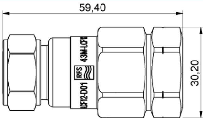
43M-LCF12-D01 Outline Drawing
