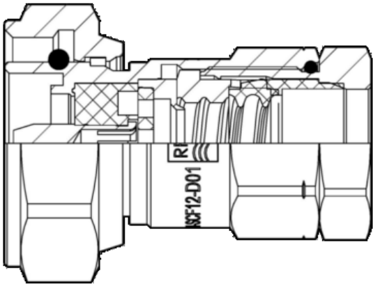
716M-SCF12-D01_DRW.png
